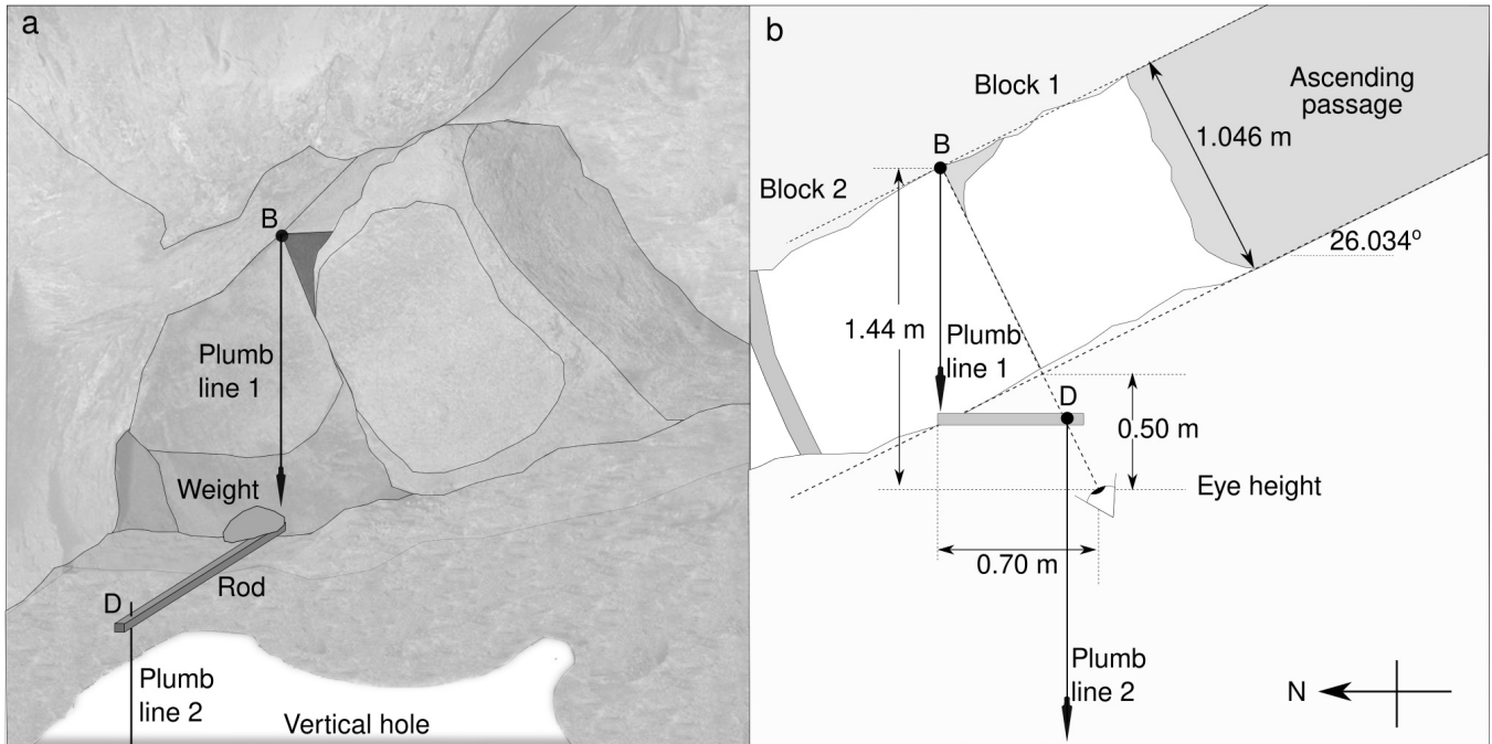
Diagram A3 - An analysis of the surveying error of Smyth
