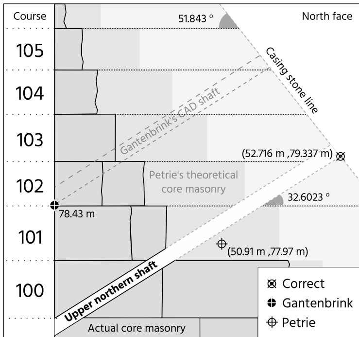
Diagram A7 - The upper northern shaft exit
