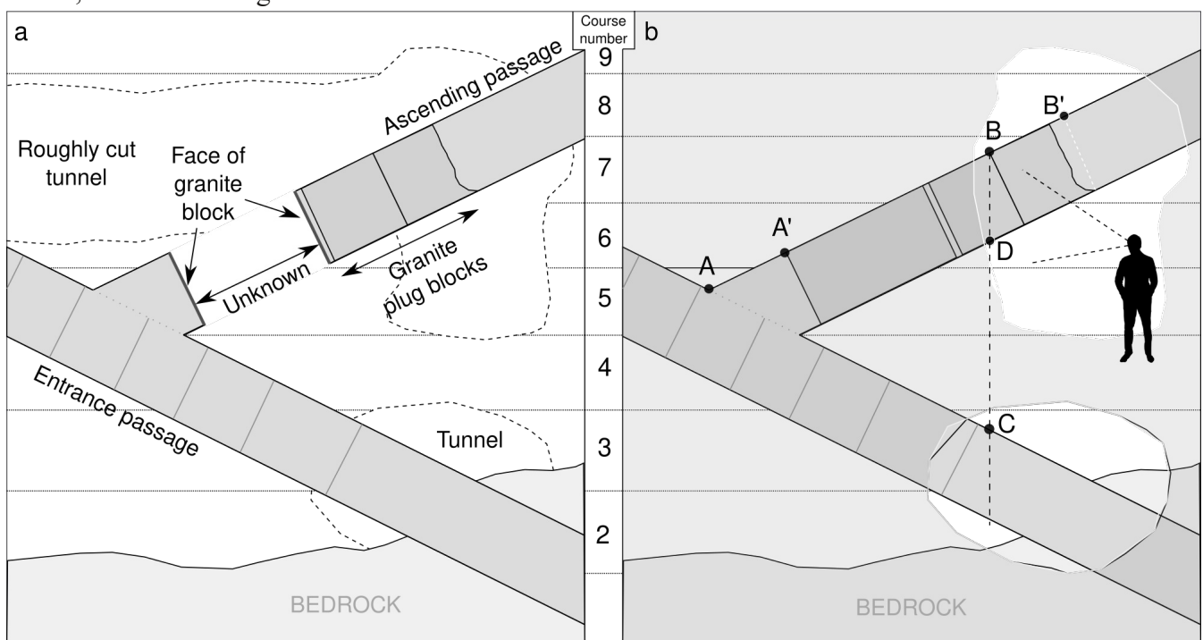
Diagram A2 - The ascending passage a) Cross section looking east b) View from inside the roughly cut tunnel
