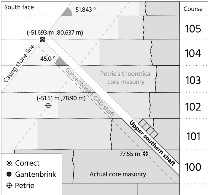
Diagram A5 - The upper southern shaft exit
