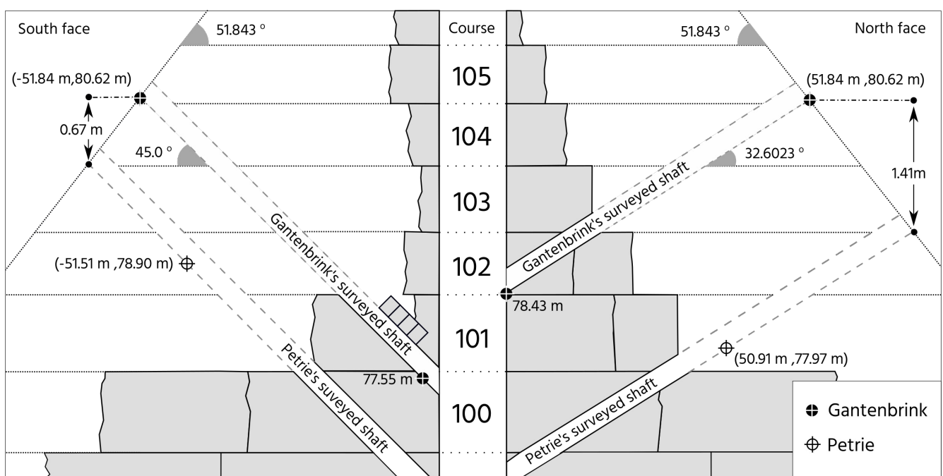
Diagram A1 - The exits of the Great Pyramid's upper shafts
