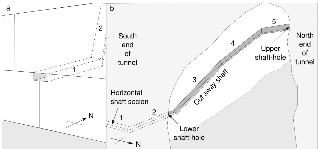
Diagram A6 - a) North wall of the upper chamber b) The tunnel at the back of the upper chamber north wall
