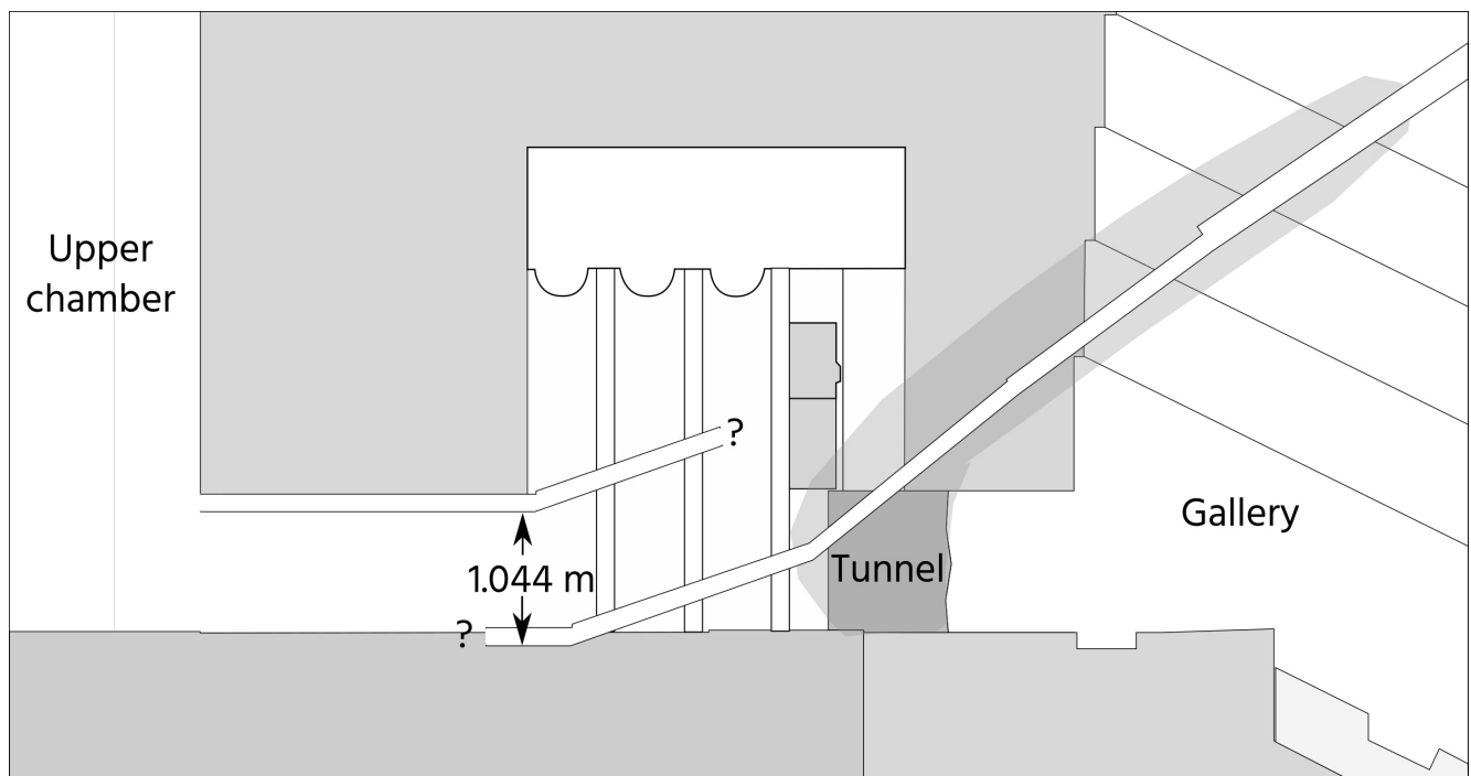
Diagram A8 - The upper chamber northern shaft and the upper northern shaft end inside the tunnel
